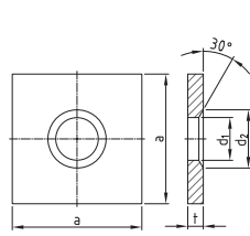
Ankerplatte Konus 30° anchor plate cone 30°
