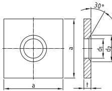
Ankerplatte Konus 30° anchor plate cone 30°
