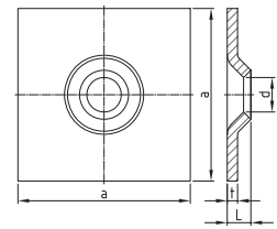
Ankerplatte ballig 30°/55° domed washer 30°/55°
