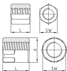
Ankermutter anchor nut
