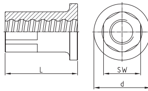
Spannverankerung stressing anchorage
