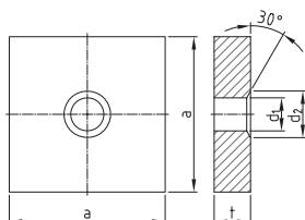
Ankerplatte Konus 30° anchor plate rectangular 30°
